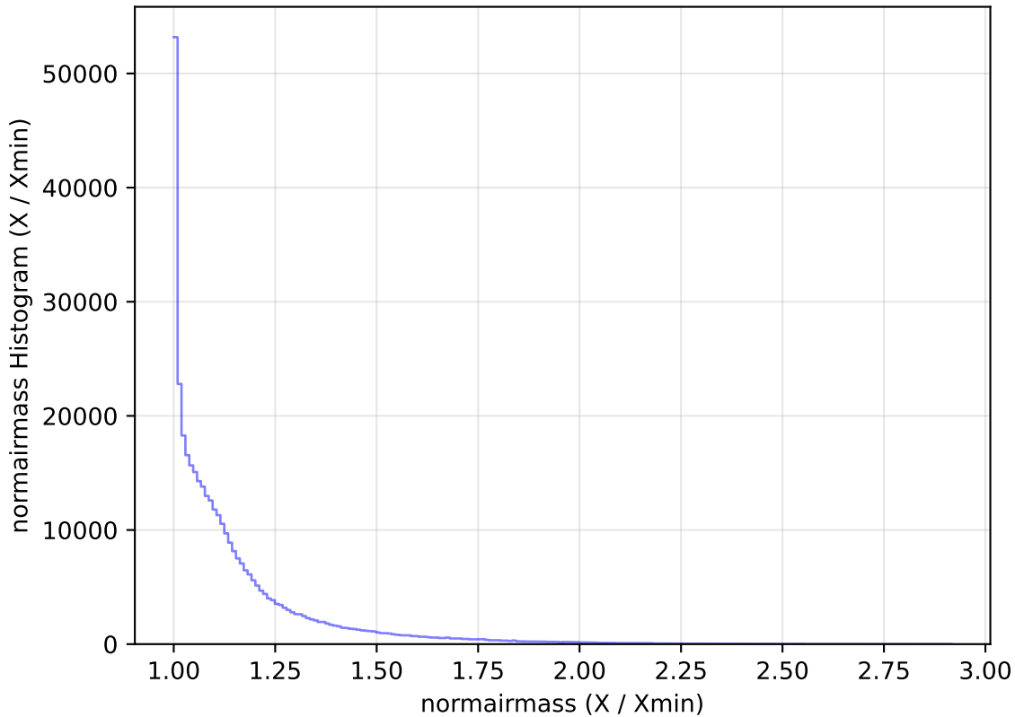
too_elab_r32_d2_giz_v3.4_10yrs WFD y band: normairmass Histogram
