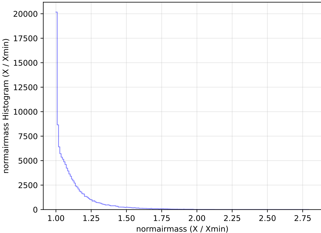
too_elab_r32_d2_giz_v3.4_10yrs WFD u band: normairmass Histogram
