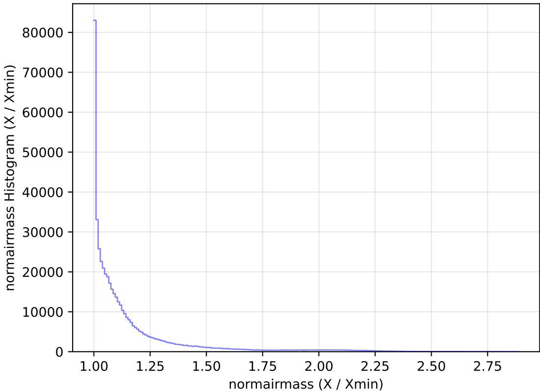
too_elab_r32_d2_giz_v3.4_10yrs WFD r band: normairmass Histogram
