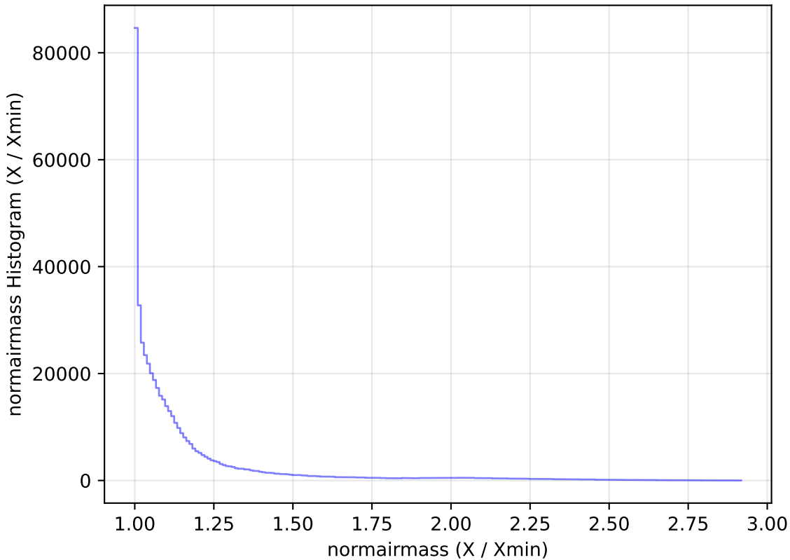
too_elab_r32_d2_giz_v3.4_10yrs WFD i band: normairmass Histogram
