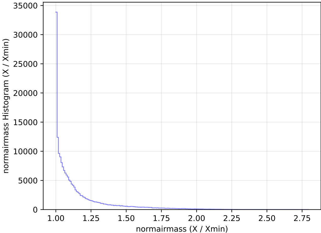
too_elab_r32_d2_giz_v3.4_10yrs WFD g band: normairmass Histogram
