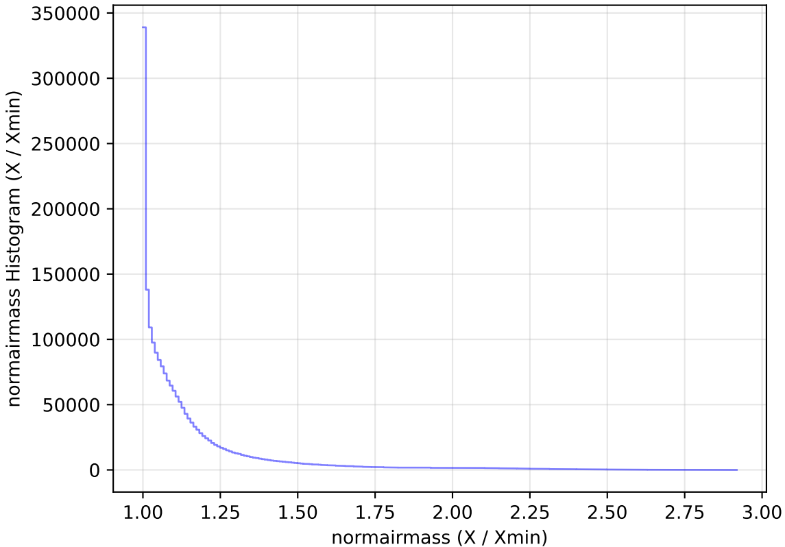
too_elab_r32_d2_giz_v3.4_10yrs WFD all bands: normairmass Histogram
