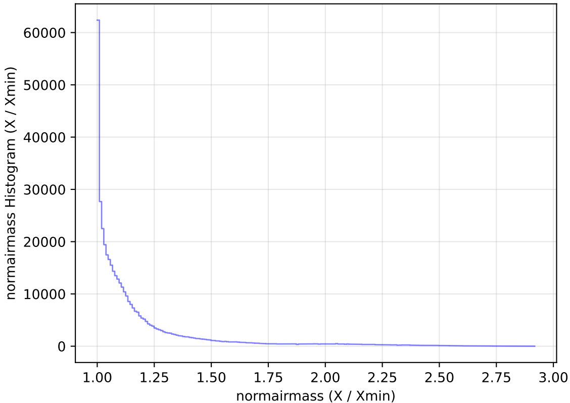
too_elab_r32_d2_giz_v3.4_10yrs All sky z band: normairmass Histogram
