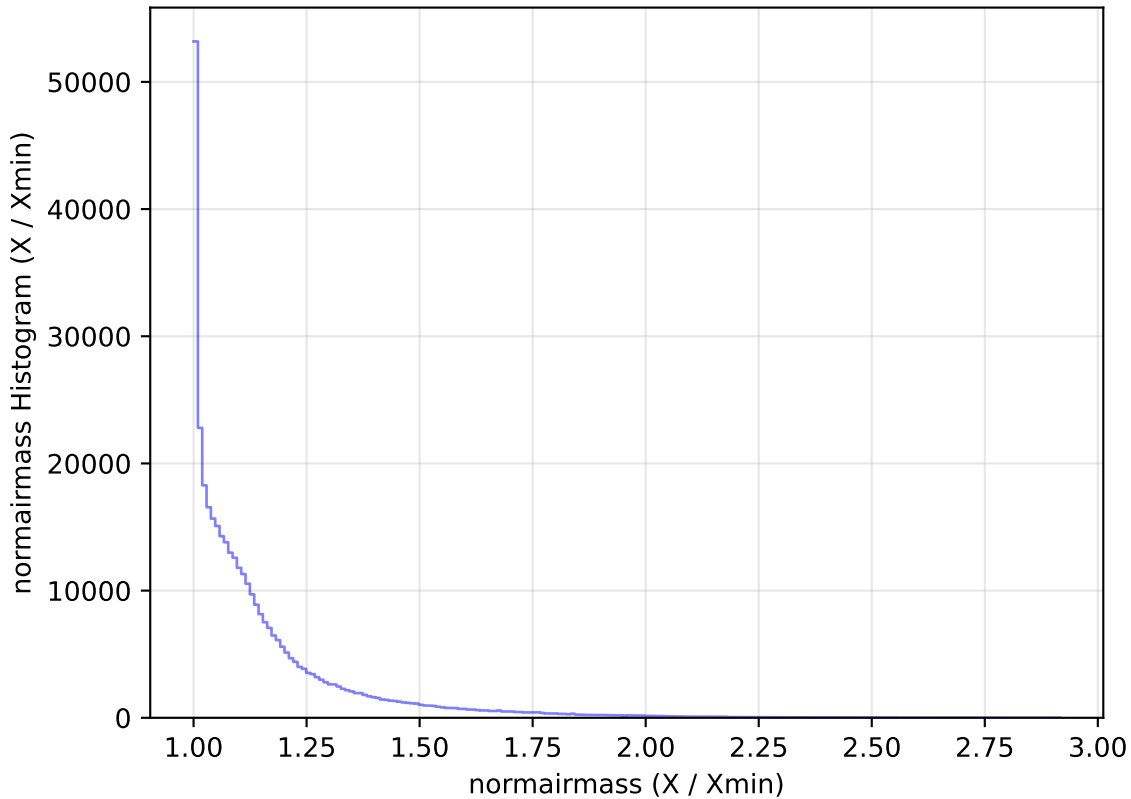
too_elab_r32_d2_giz_v3.4_10yrs All sky y band: normairmass Histogram
