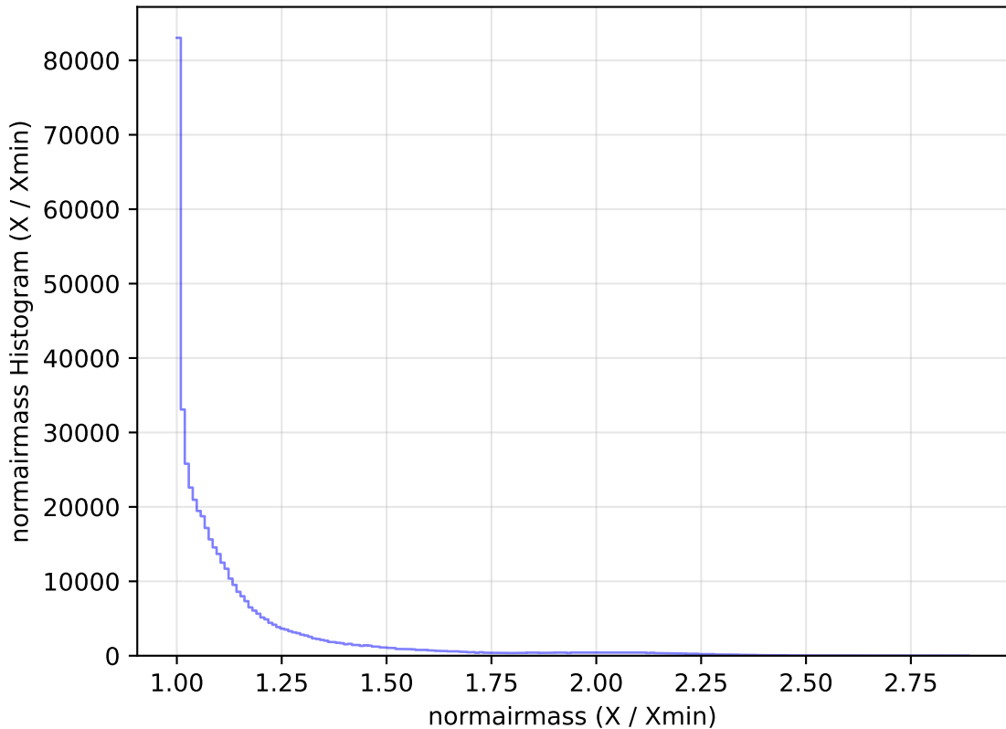
too_elab_r32_d2_giz_v3.4_10yrs All sky r band: normairmass Histogram
