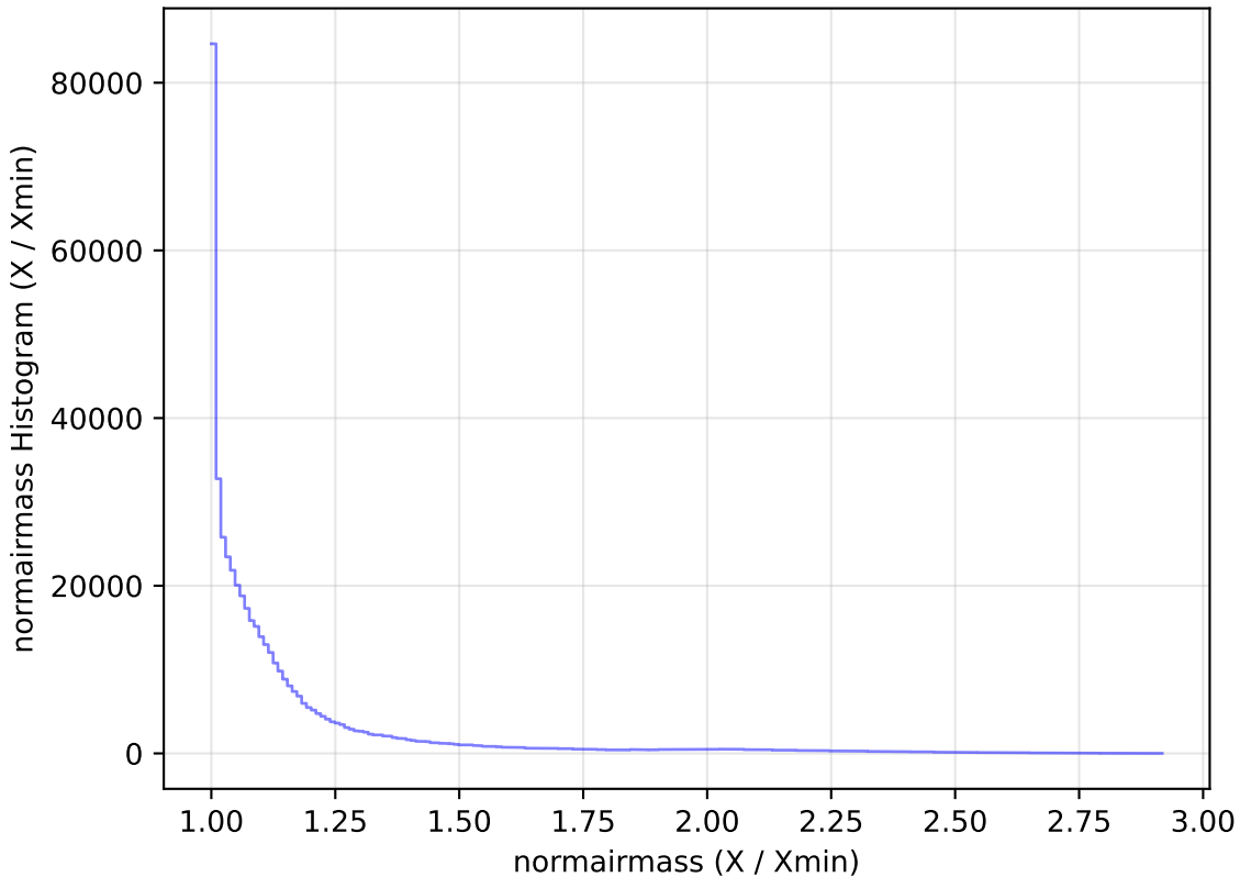
too_elab_r32_d2_giz_v3.4_10yrs All sky i band: normairmass Histogram
