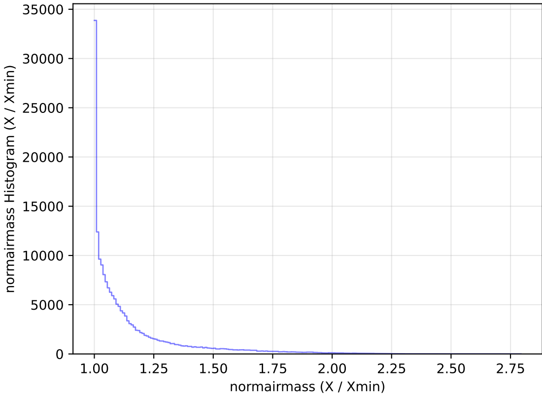
too_elab_r32_d2_giz_v3.4_10yrs All sky g band: normairmass Histogram
