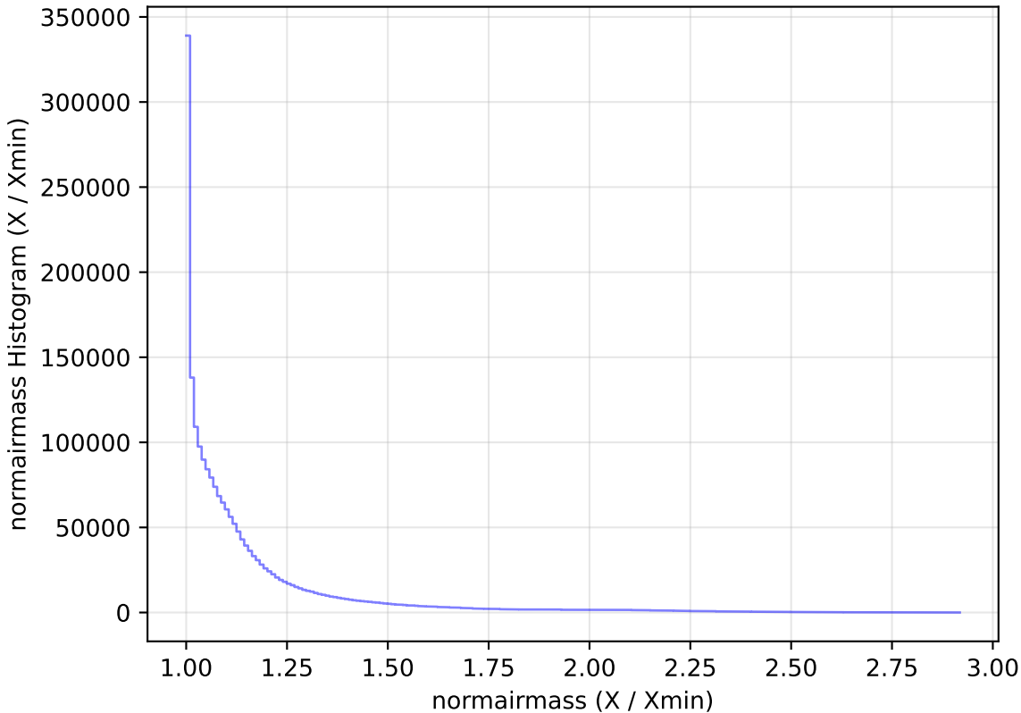
too_elab_r32_d2_giz_v3.4_10yrs All sky all bands: normairmass Histogram
