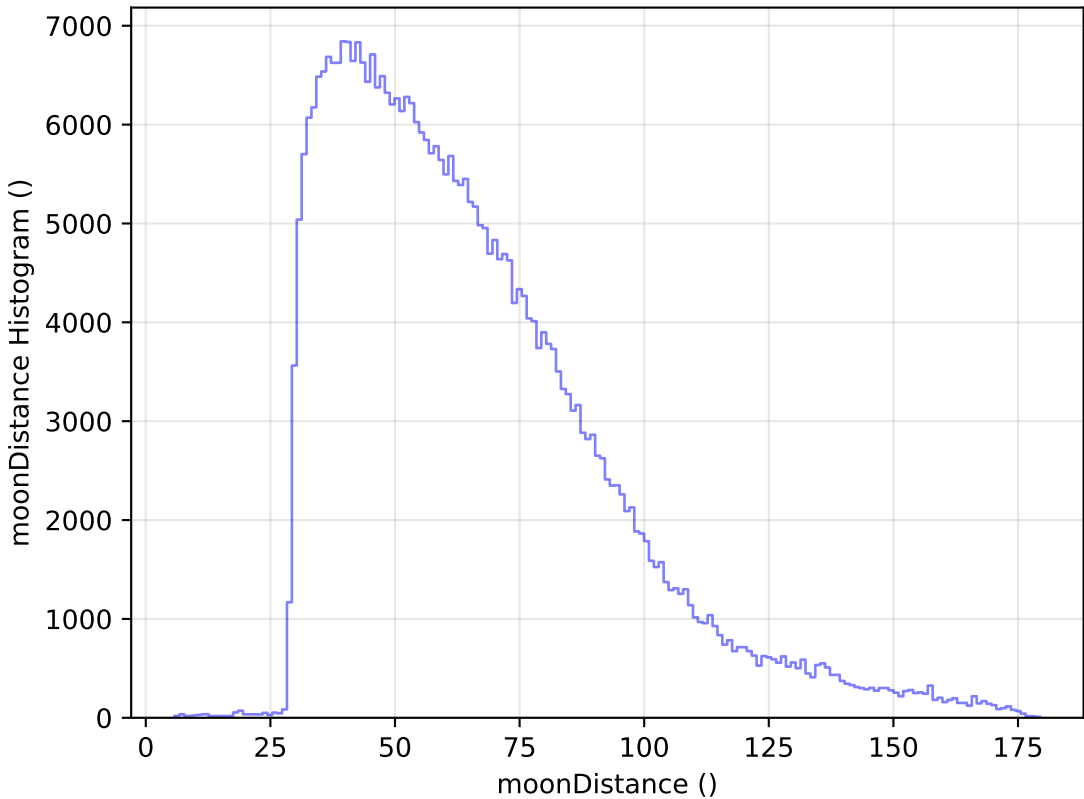
too_elab_r32_d2_giz_v3.4_10yrs WFD y band: moonDistance Histogram
