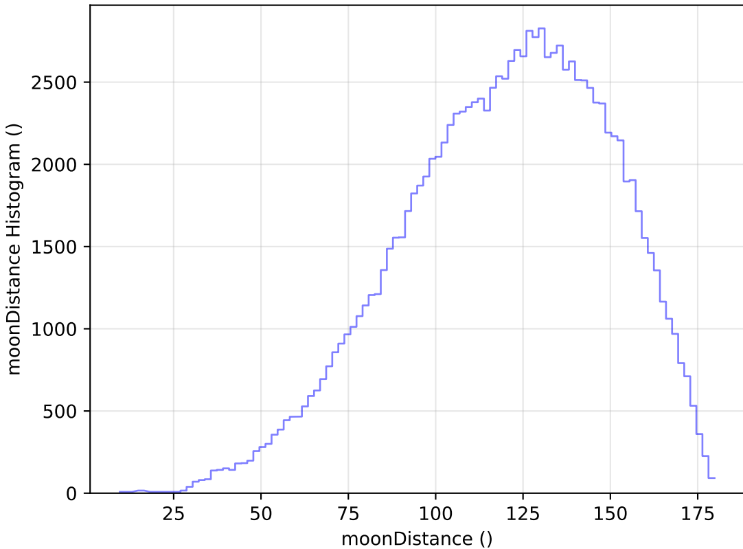
too_elab_r32_d2_giz_v3.4_10yrs WFD u band: moonDistance Histogram
