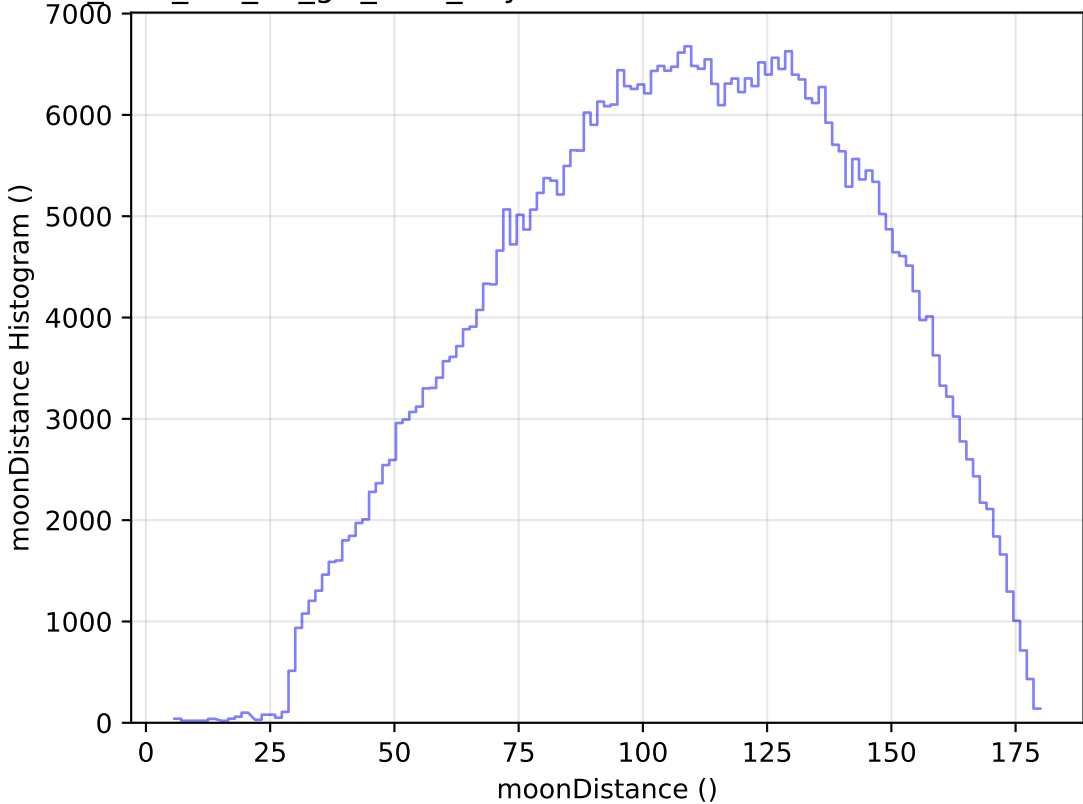
too_elab_r32_d2_giz_v3.4_10yrs WFD r band: moonDistance Histogram
