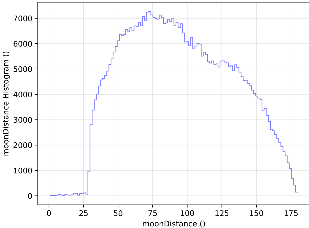
too_elab_r32_d2_giz_v3.4_10yrs WFD i band: moonDistance Histogram
