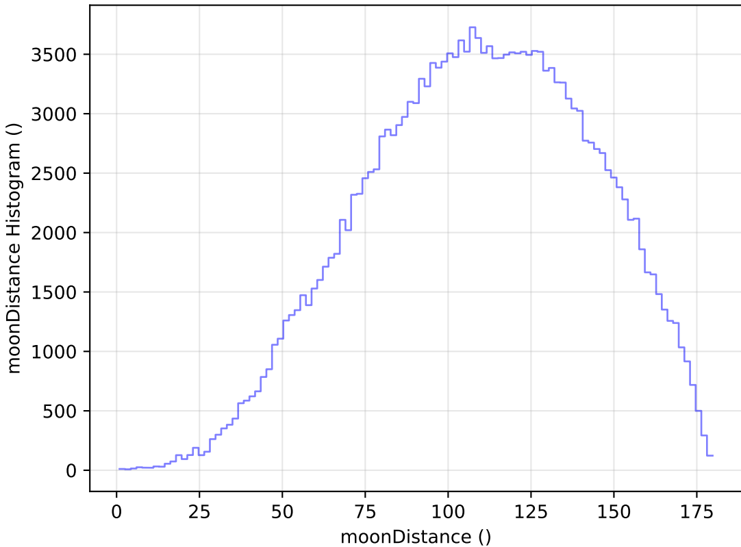
too_elab_r32_d2_giz_v3.4_10yrs WFD g band: moonDistance Histogram
