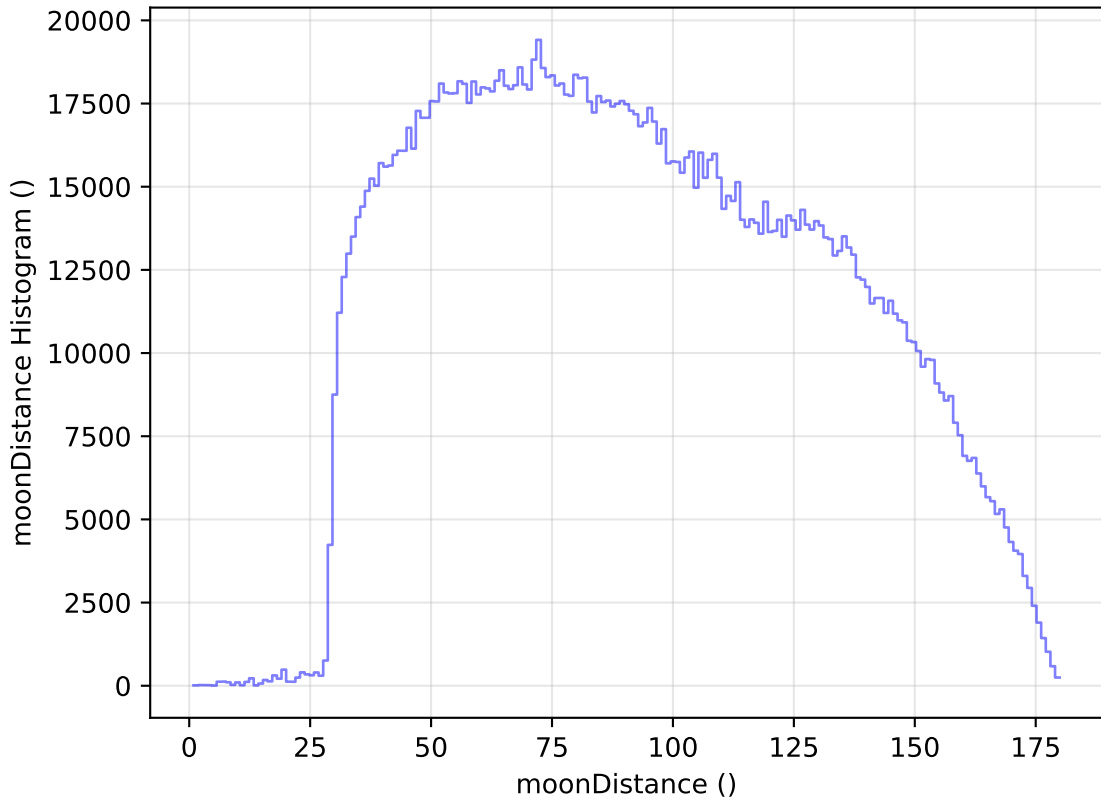
too_elab_r32_d2_giz_v3.4_10yrs WFD all bands: moonDistance Histogram
