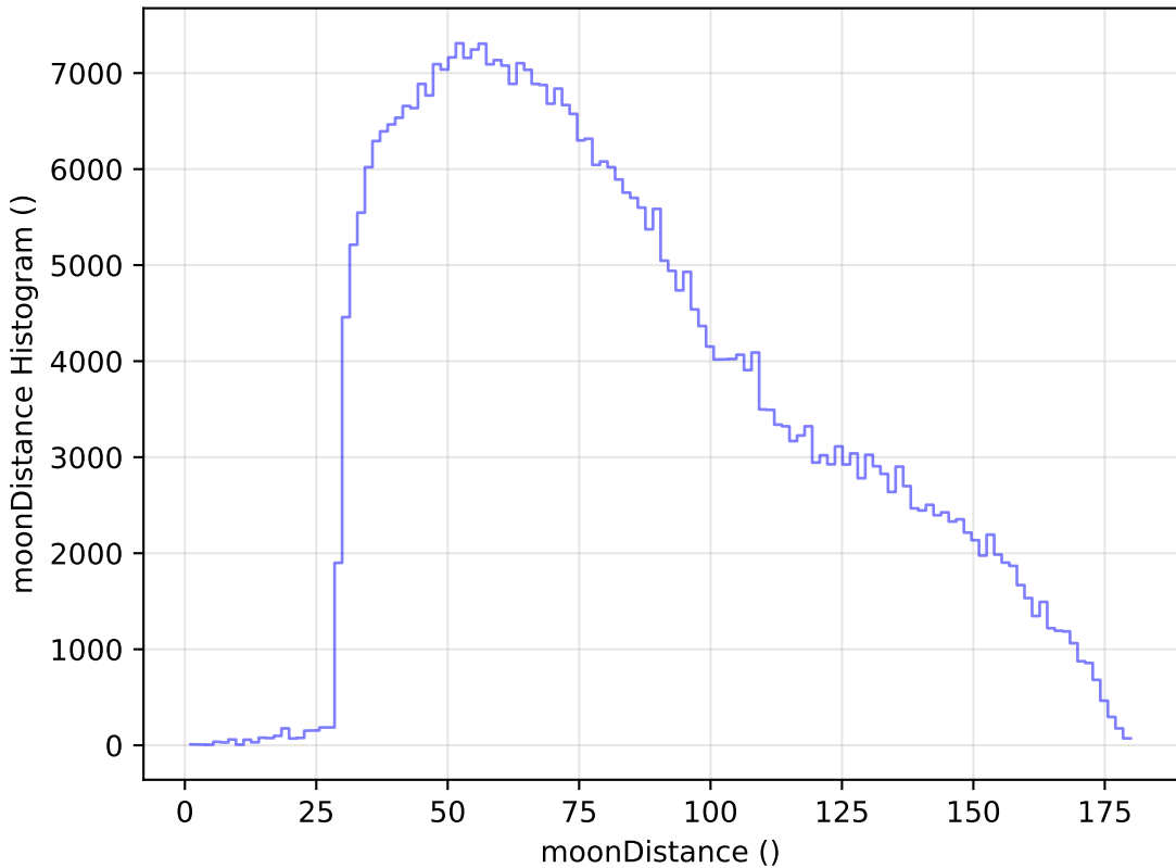
too_elab_r32_d2_giz_v3.4_10yrs All sky z band: moonDistance Histogram
