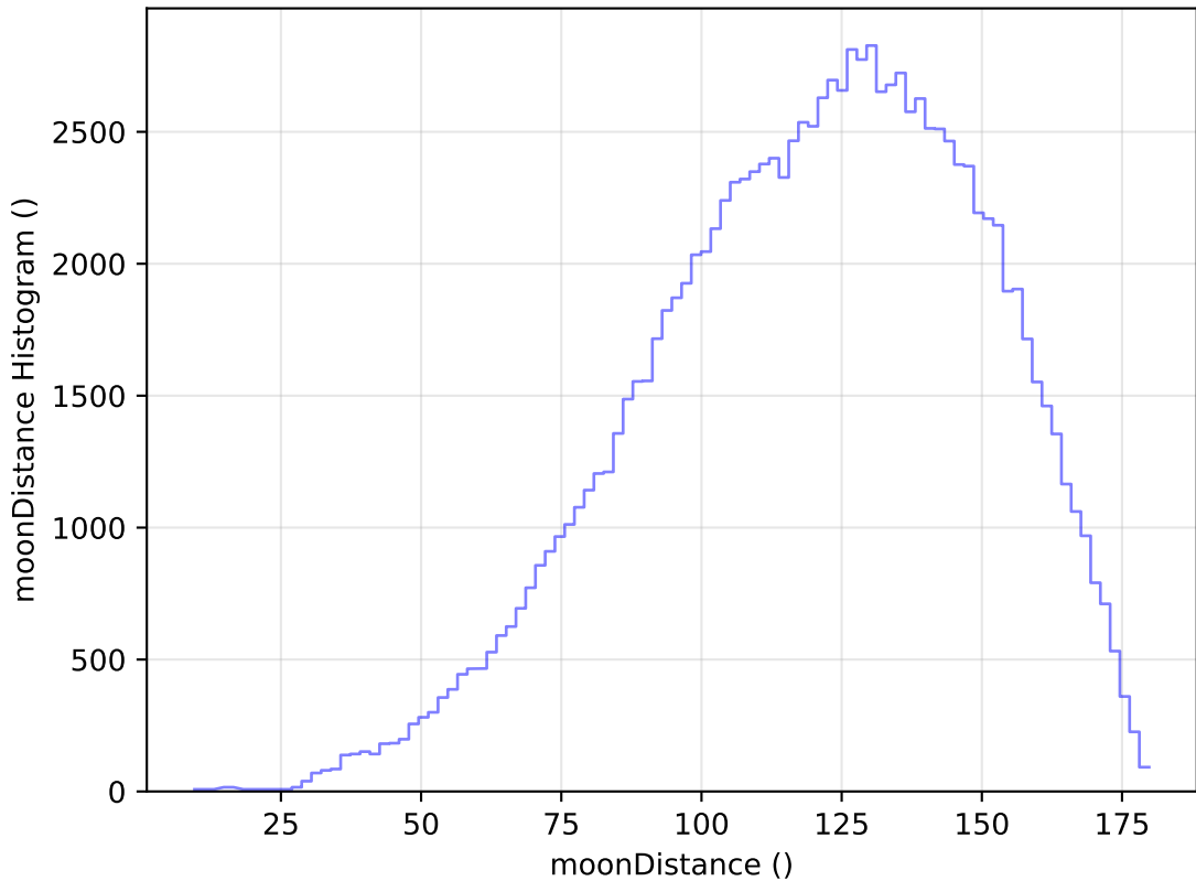
too_elab_r32_d2_giz_v3.4_10yrs All sky u band: moonDistance Histogram
