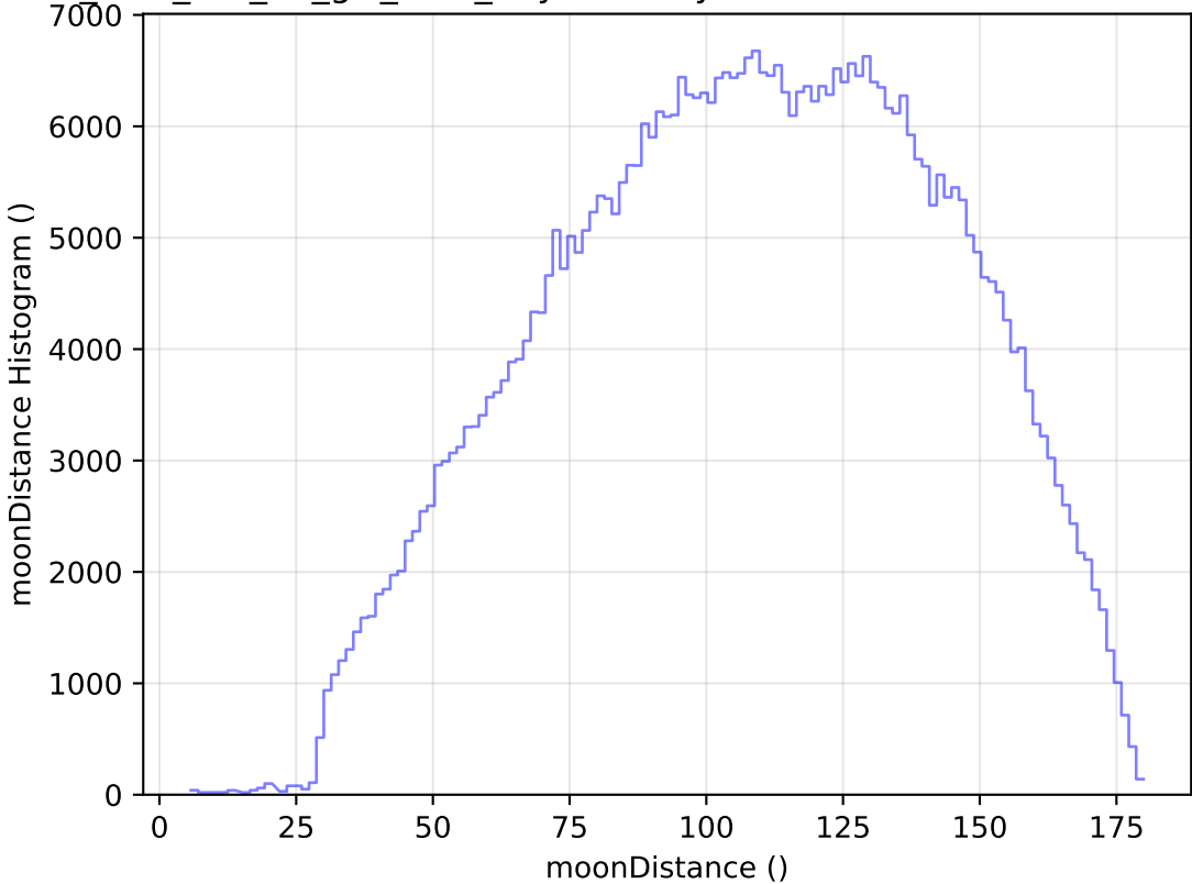
too_elab_r32_d2_giz_v3.4_10yrs All sky r band: moonDistance Histogram
