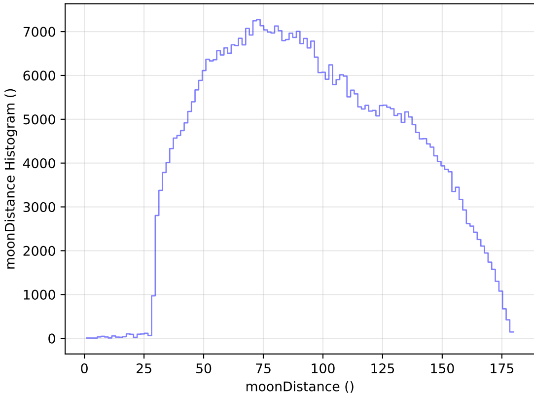
too_elab_r32_d2_giz_v3.4_10yrs All sky i band: moonDistance Histogram
