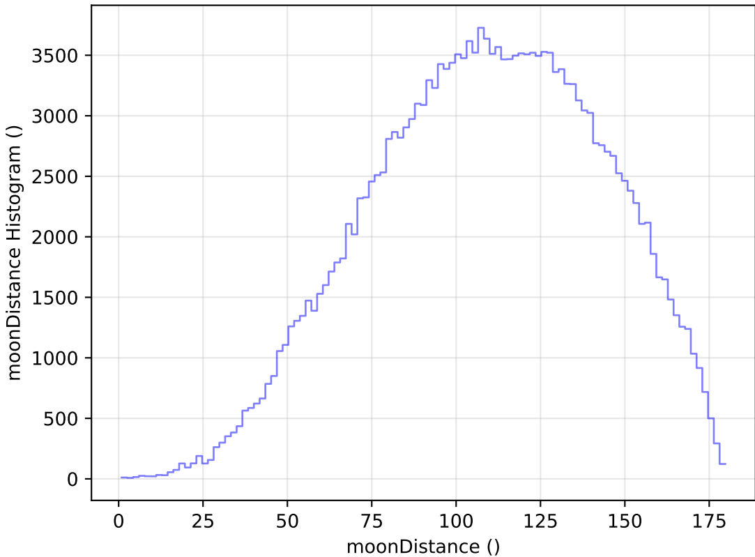
too_elab_r32_d2_giz_v3.4_10yrs All sky g band: moonDistance Histogram
