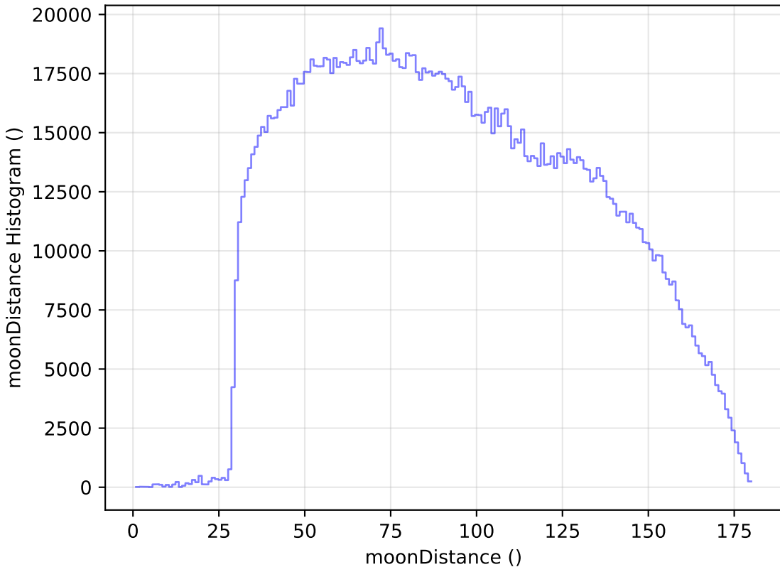
too_elab_r32_d2_giz_v3.4_10yrs All sky all bands: moonDistance Histogram
