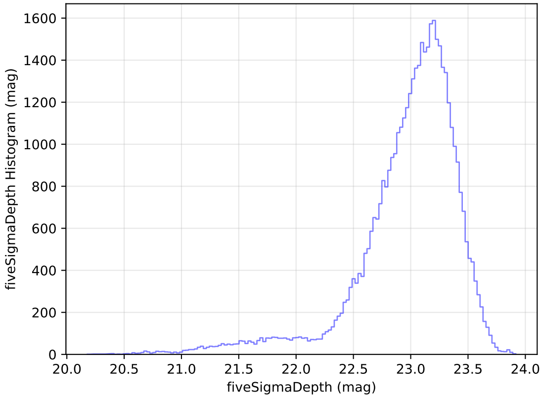
too_elab_r32_d2_giz_v3.4_10yrs Yr 1 z band: fiveSigmaDepth Histogram
