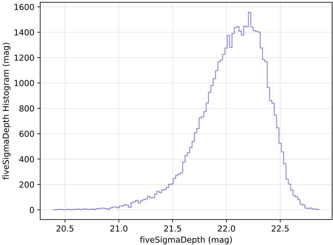
too_elab_r32_d2_giz_v3.4_10yrs Yr 1 y band: fiveSigmaDepth Histogram
