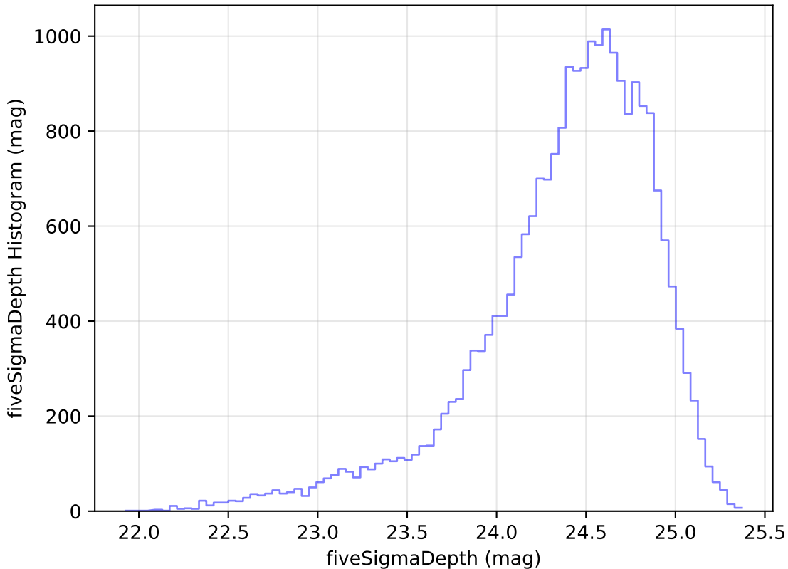
too_elab_r32_d2_giz_v3.4_10yrs Yr 1 g band: fiveSigmaDepth Histogram
