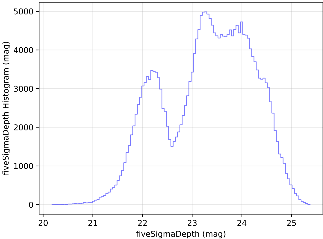
too_elab_r32_d2_giz_v3.4_10yrs Yr 1 all bands: fiveSigmaDepth Histogram
