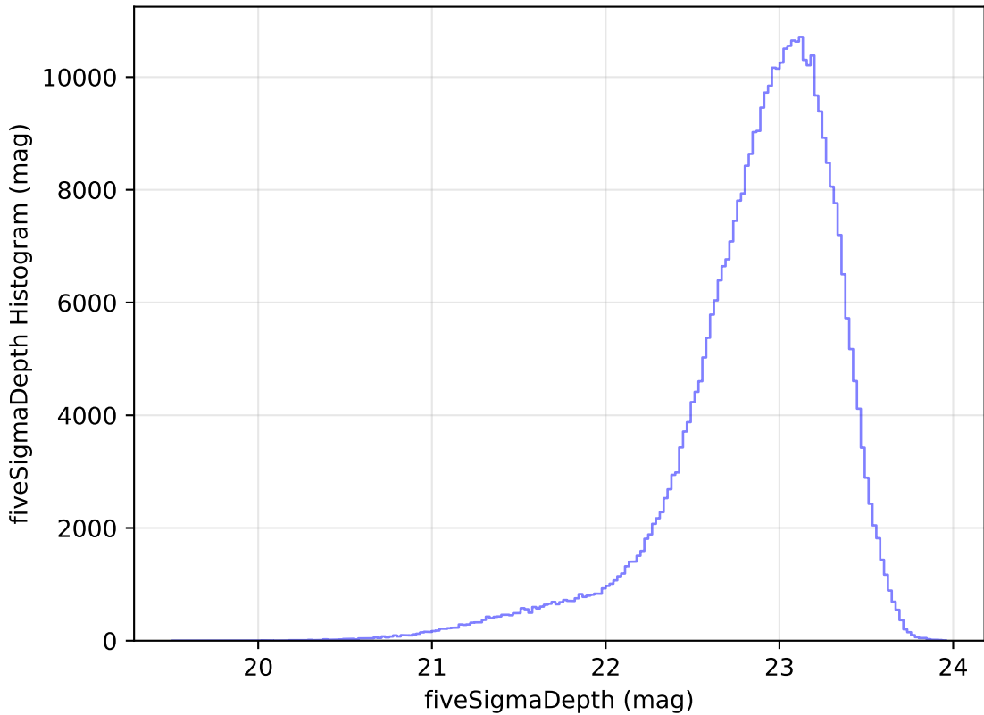
too_elab_r32_d2_giz_v3.4_10yrs WFD z band: fiveSigmaDepth Histogram
