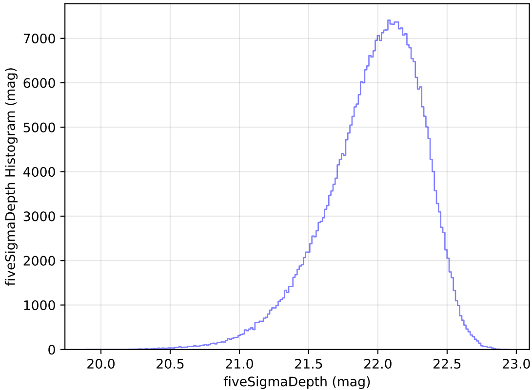
too_elab_r32_d2_giz_v3.4_10yrs WFD y band: fiveSigmaDepth Histogram
