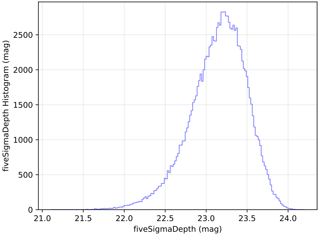
too_elab_r32_d2_giz_v3.4_10yrs WFD u band: fiveSigmaDepth Histogram
