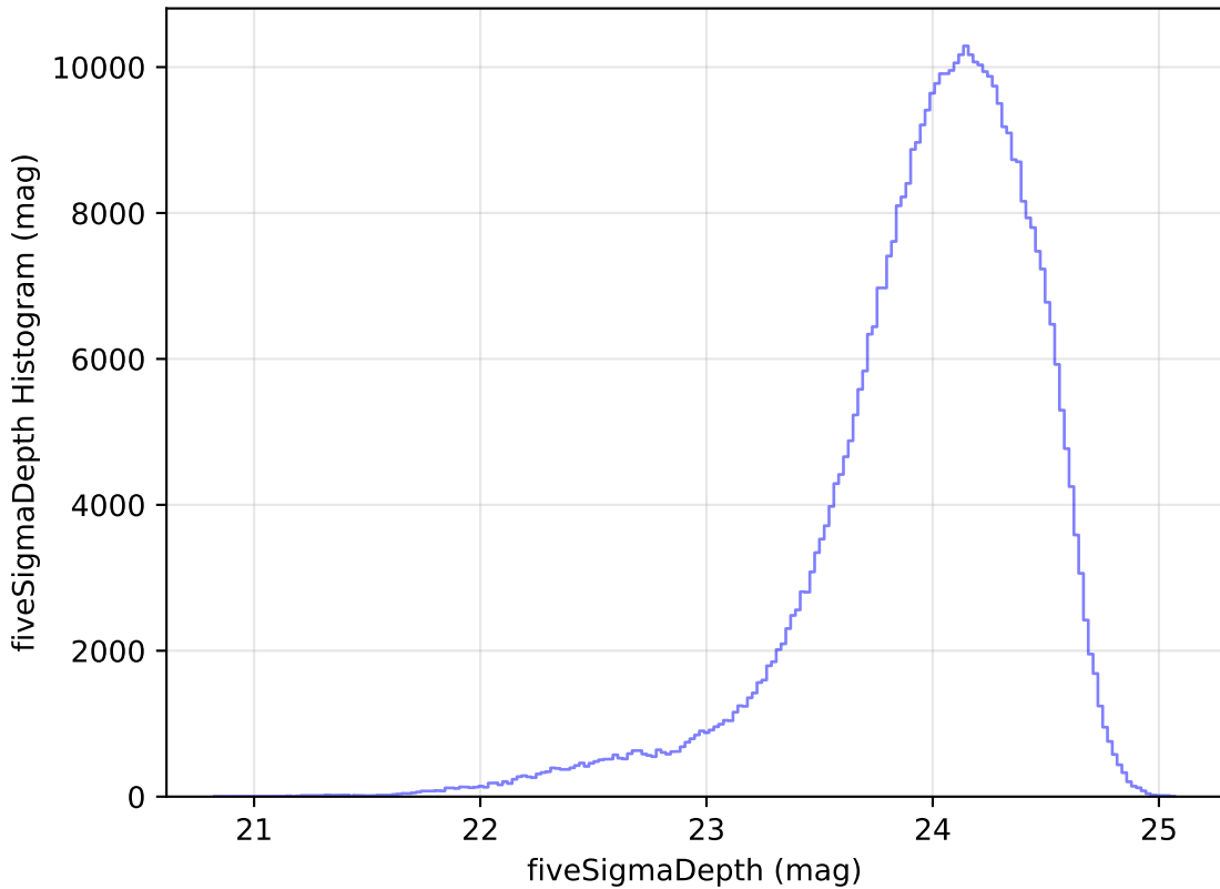
too_elab_r32_d2_giz_v3.4_10yrs WFD r band: fiveSigmaDepth Histogram
