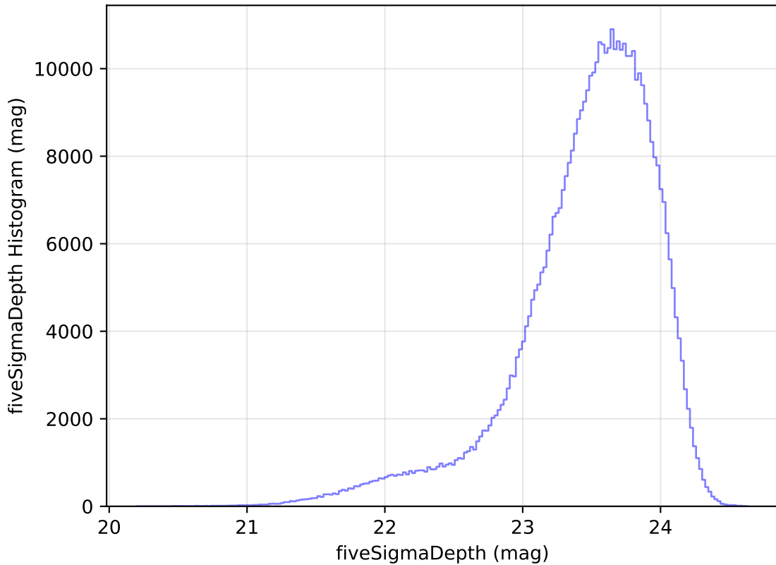
too_elab_r32_d2_giz_v3.4_10yrs WFD i band: fiveSigmaDepth Histogram
