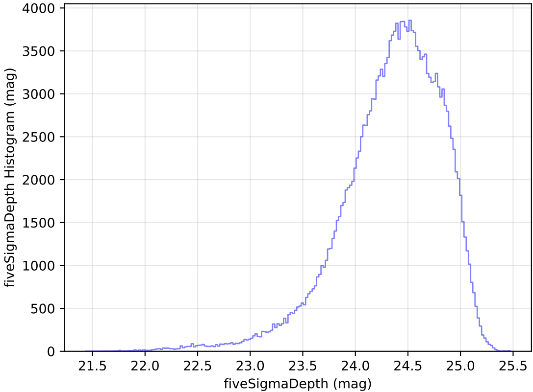
too_elab_r32_d2_giz_v3.4_10yrs WFD g band: fiveSigmaDepth Histogram
