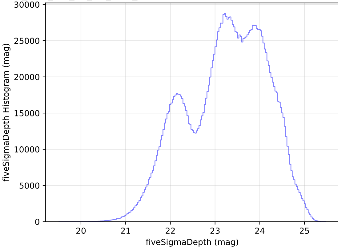
too_elab_r32_d2_giz_v3.4_10yrs WFD all bands: fiveSigmaDepth Histogram
