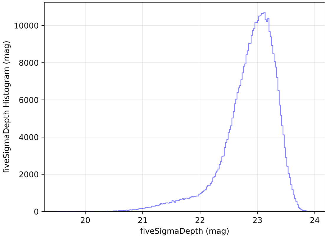
too_elab_r32_d2_giz_v3.4_10yrs All sky z band: fiveSigmaDepth Histogram
