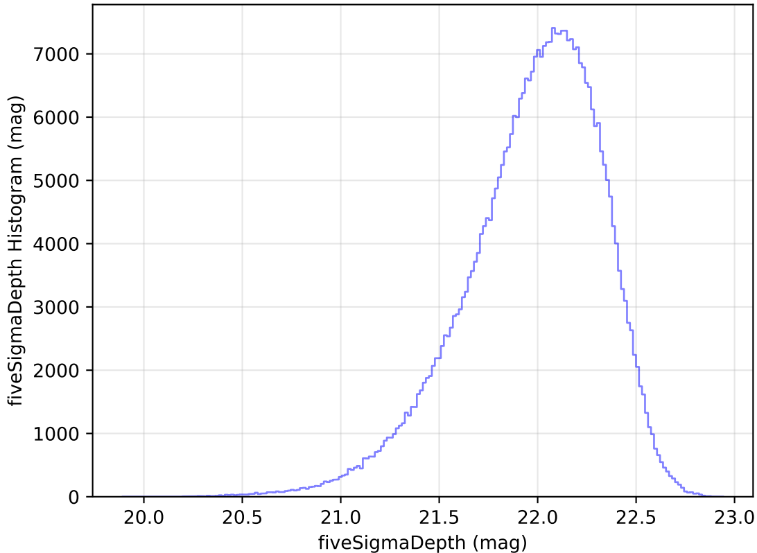
too_elab_r32_d2_giz_v3.4_10yrs All sky y band: fiveSigmaDepth Histogram
