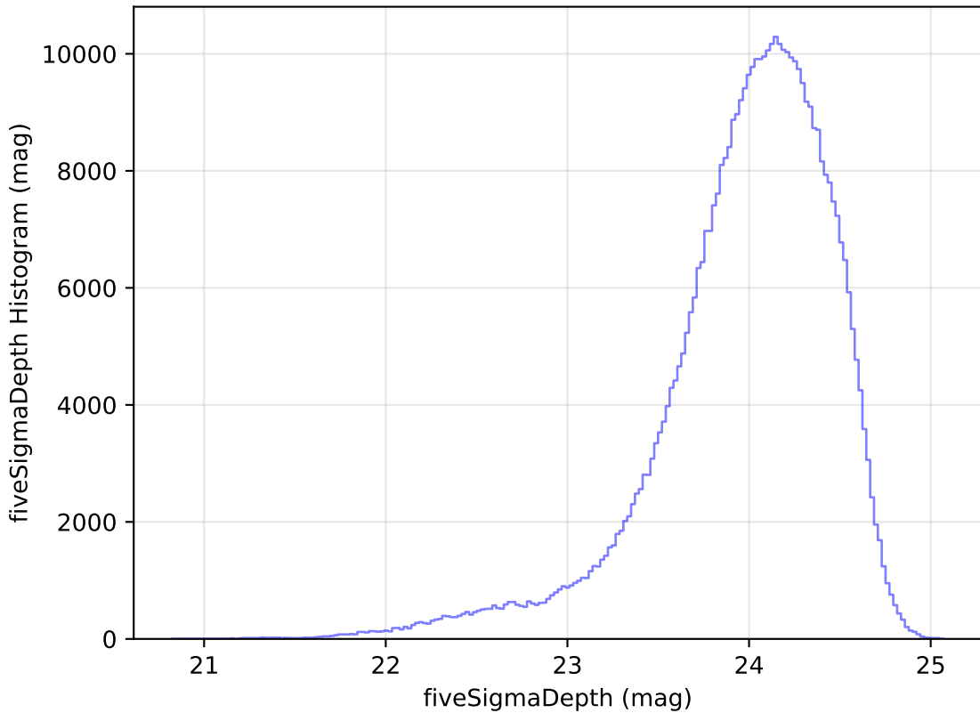
too_elab_r32_d2_giz_v3.4_10yrs All sky r band: fiveSigmaDepth Histogram
