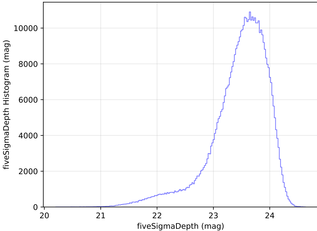
too_elab_r32_d2_giz_v3.4_10yrs All sky i band: fiveSigmaDepth Histogram
