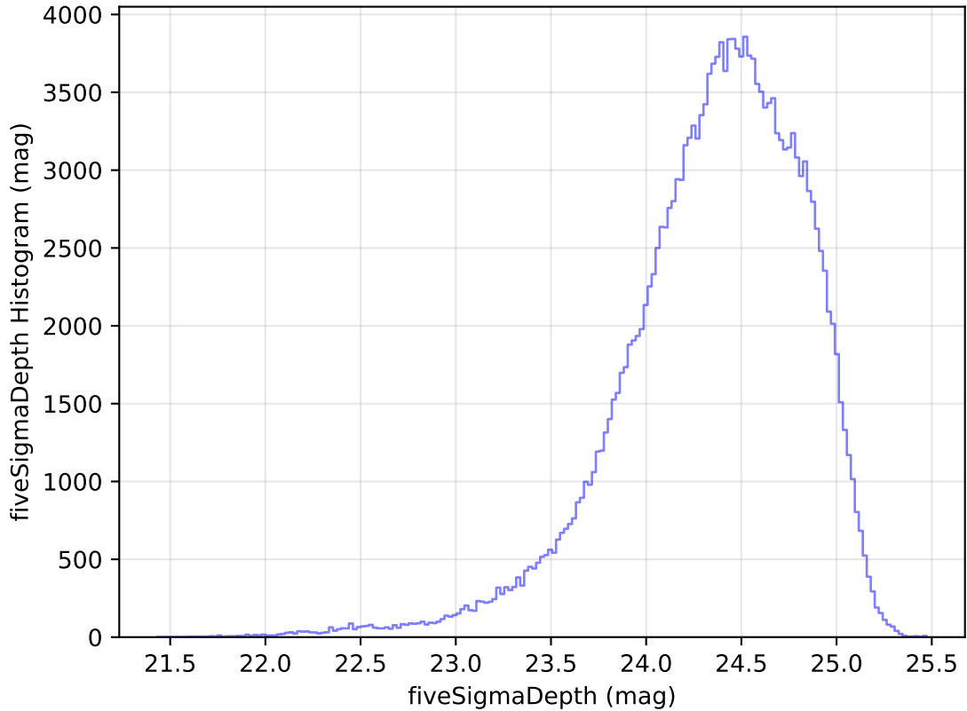
too_elab_r32_d2_giz_v3.4_10yrs All sky g band: fiveSigmaDepth Histogram
