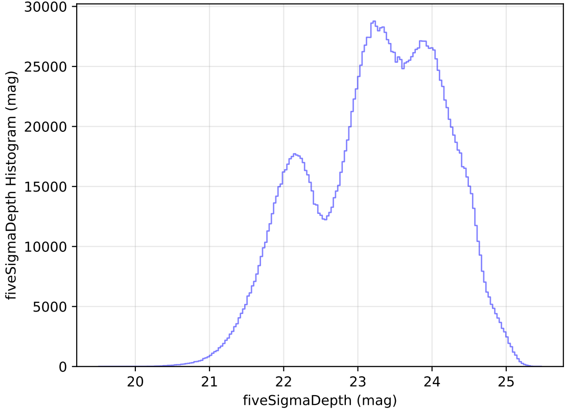
too_elab_r32_d2_giz_v3.4_10yrs All sky all bands: fiveSigmaDepth Histogram
