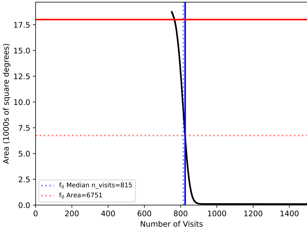
too_elab_r32_d2_giz_v3.4_10yrs WFD: f0
