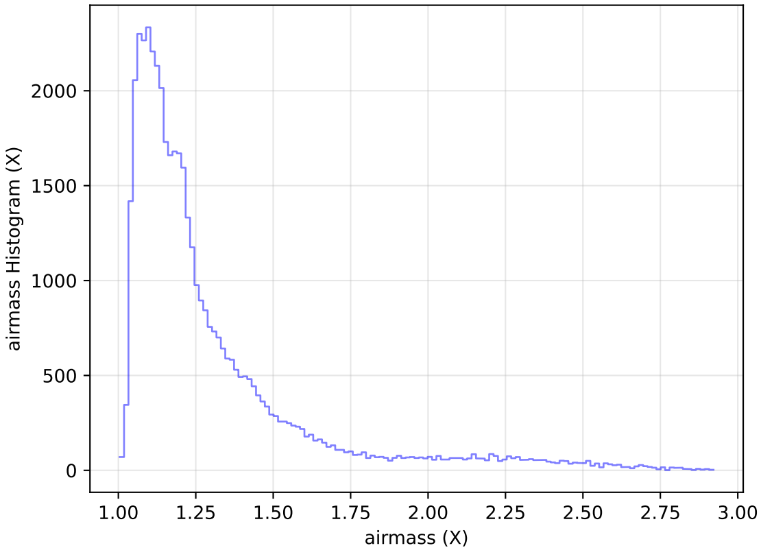
too_elab_r32_d2_giz_v3.4_10yrs Yr 1 z band: airmass Histogram
