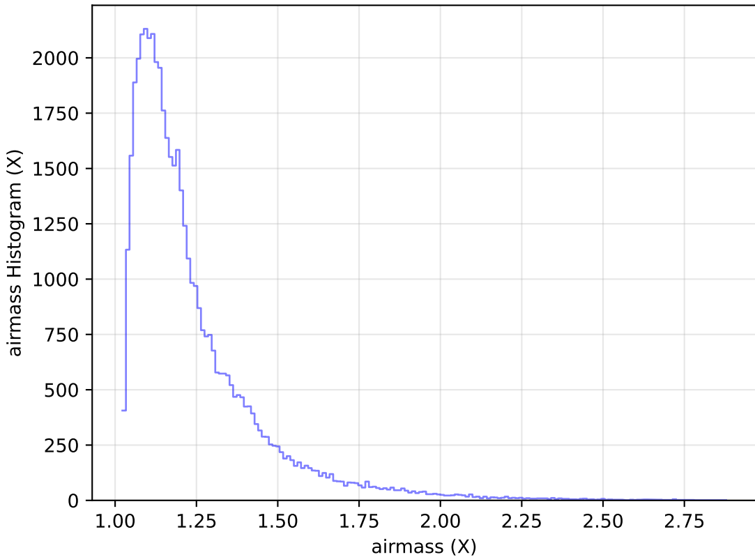
too_elab_r32_d2_giz_v3.4_10yrs Yr 1 y band: airmass Histogram
