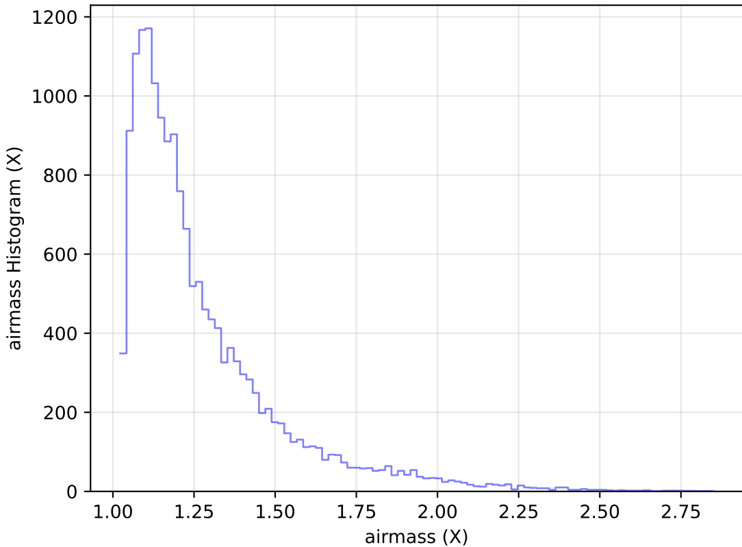
too_elab_r32_d2_giz_v3.4_10yrs Yr 1 u band: airmass Histogram
