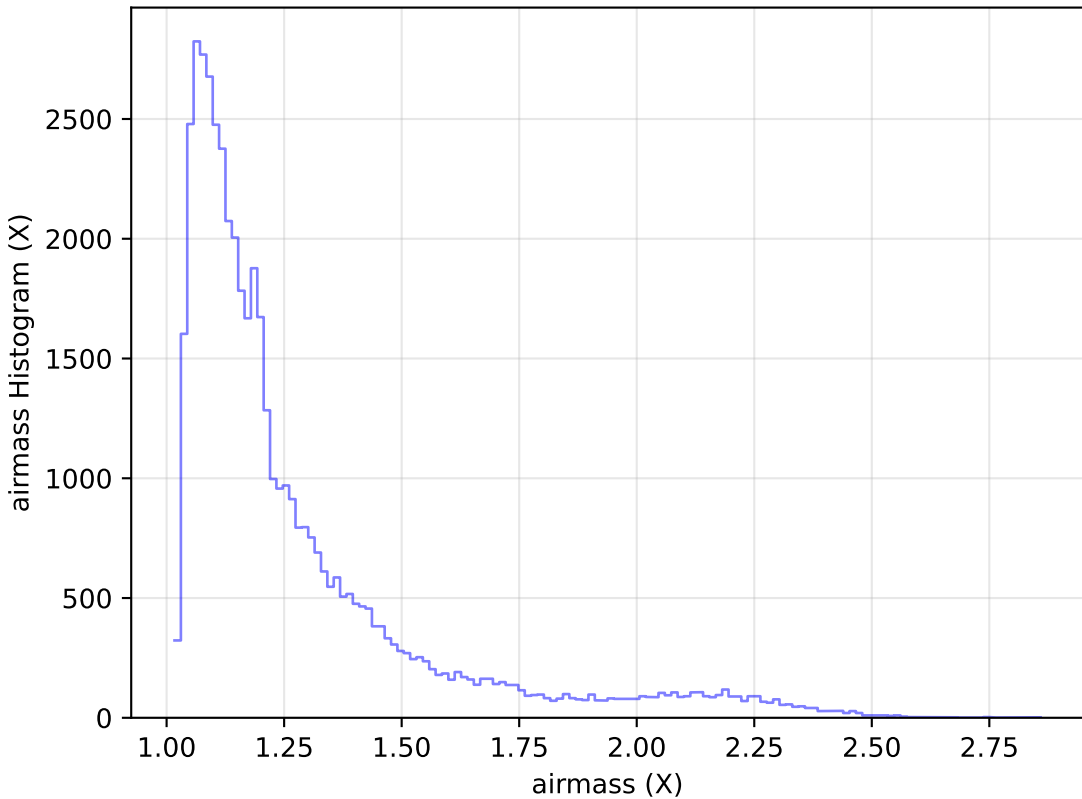
too_elab_r32_d2_giz_v3.4_10yrs Yr 1 r band: airmass Histogram
