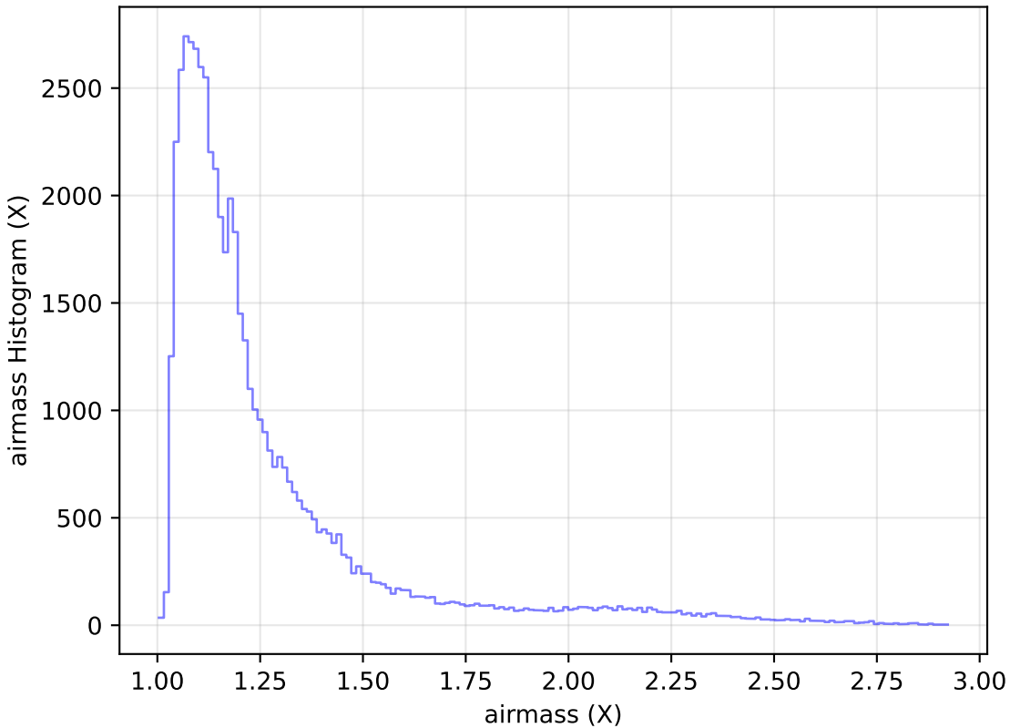
too_elab_r32_d2_giz_v3.4_10yrs Yr 1 i band: airmass Histogram
