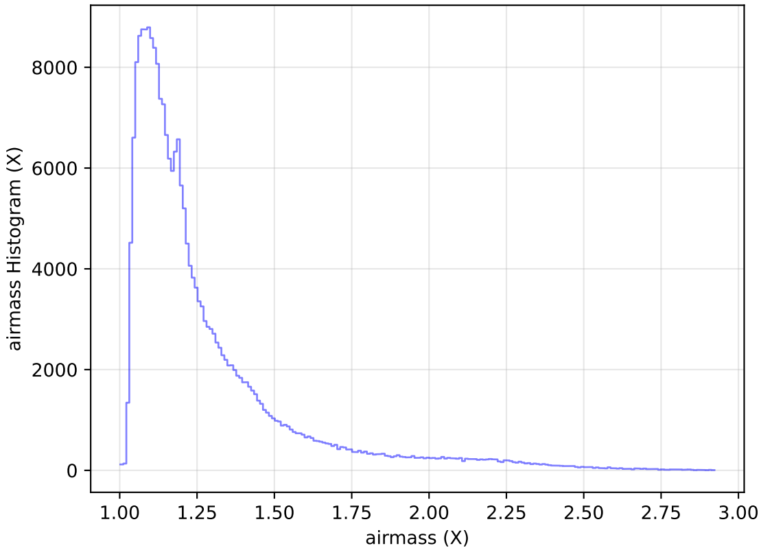
too_elab_r32_d2_giz_v3.4_10yrs Yr 1 all bands: airmass Histogram
