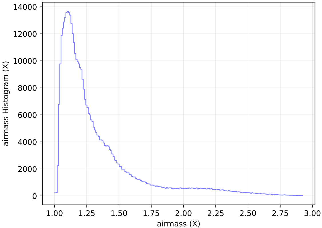
too_elab_r32_d2_giz_v3.4_10yrs WFD z band: airmass Histogram
