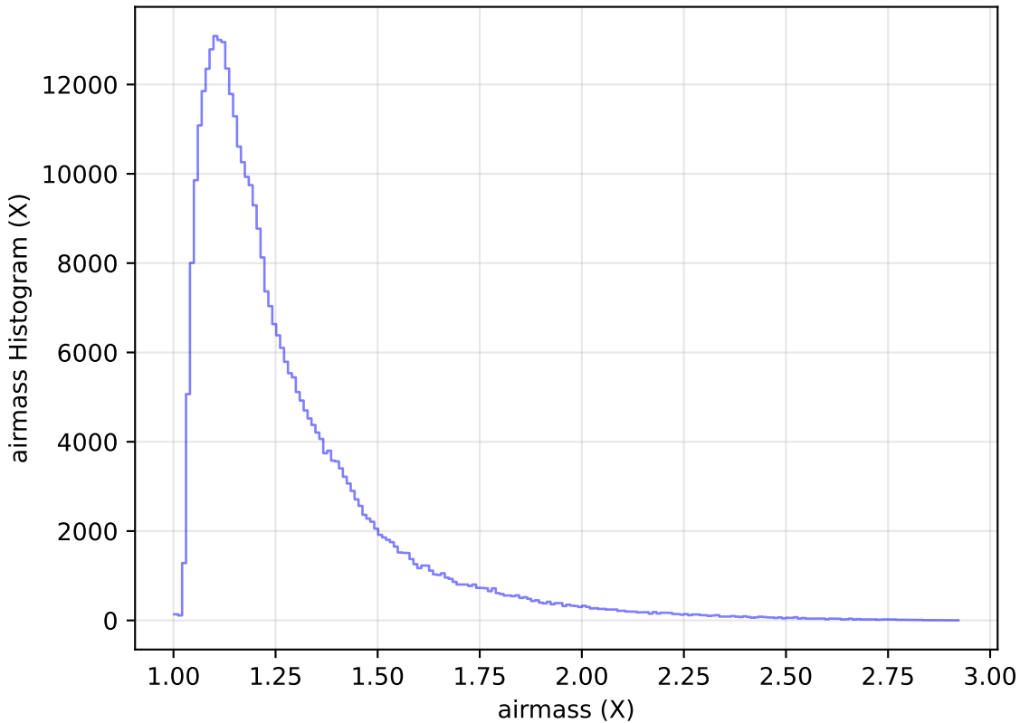
too_elab_r32_d2_giz_v3.4_10yrs WFD y band: airmass Histogram
